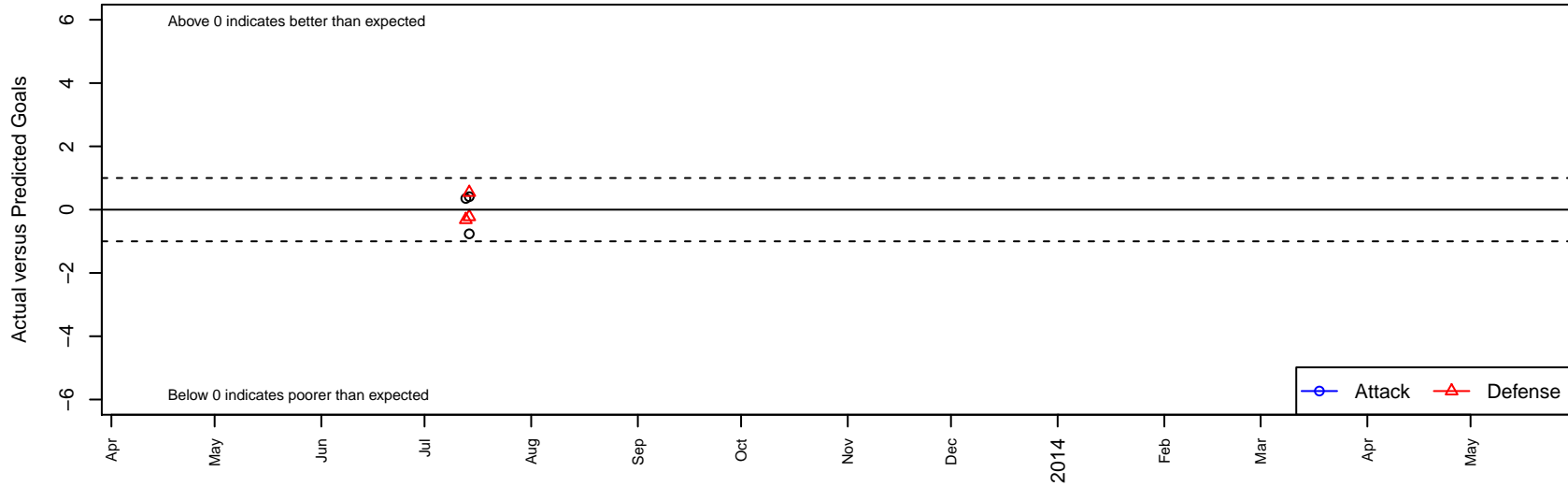
Mountain View Blue B96 Dots are actual minus expected GF (blue circles) and GA (red triangles). Blue line is smoothed change in attack strength. Red is smoothed change in defense strength.
